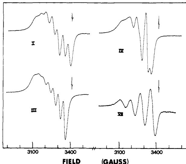
Figure 3. Room-temperature X-band EPR spectra for toluene-acetone (3:2) solutions of mixed-valence \text{Cu}^{\text{II}}\text{Cu}^{\text{I}} complexes I, III, IV, and VII. The small sharp signal superimposed above each spectrum is that for a DPPH standard.
