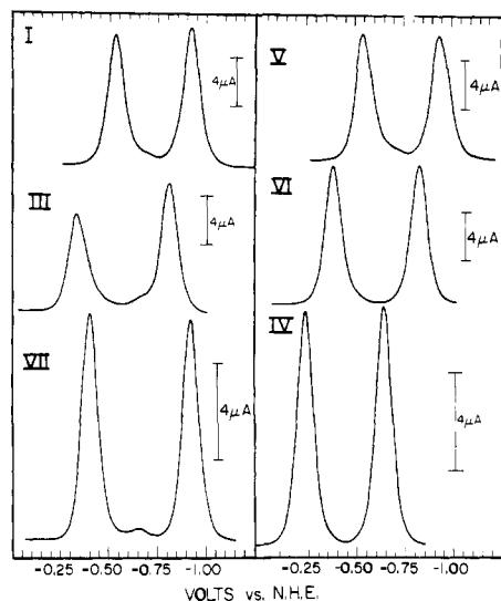
Figure 2. Differential pulse voltammograms of six of the binuclear Cu II Cu II complexes in DMF at a scan rate of 2 mV/s.
