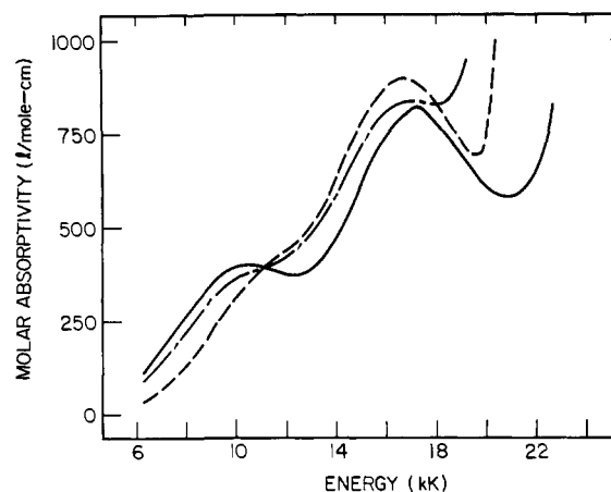
Figure 13. Electronic absorption spectra at room temperature for mixed-valence Cu II Cu I complexes I (—), IV (---), and VI (· · ·) in acetone.
