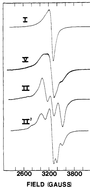
Figure 11. Liquid-helium-temperature X-band EPR spectra for solid samples of the \text{BF}_4^- salt mixed-valence complexes I, II, and V and for a solid sample of the \text{BPh}_4^- salt of the cation in complex II.
