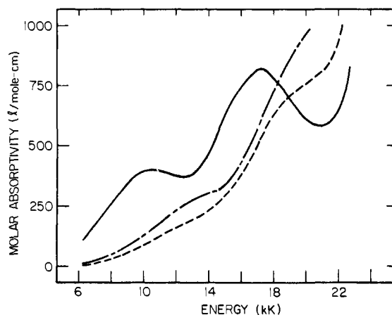
Figure 12. Electronic absorption spectra at room temperature for mixed-valence Cu II Cu I complexes I (—), III (---), and VII (· · ·) in acetone.
